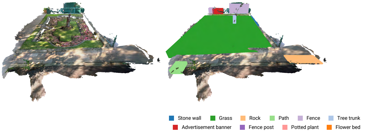
Figure 3: Results of the 3D scene understanding module. For each of the three scans— Vase , House , and Garden —we visualize the input point cloud (left) and the final set of labeled 3D bounding boxes inferred by our scene understanding pipeline (right). We also report the total time (in minutes) required to estimate the scene graph for each scan. Note that some bounding boxes may be enclosed within others and may therefore be occluded.
